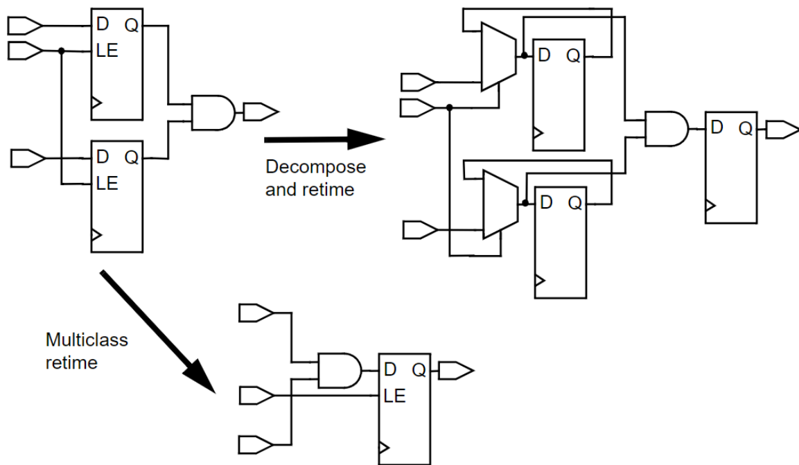
Figure 142 Reduced Area Through Multiclass Retiming
