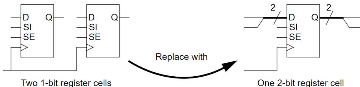
Figure 92 Replacing Multiple Single-Bit Register Cells With a Multibit Register Cell
