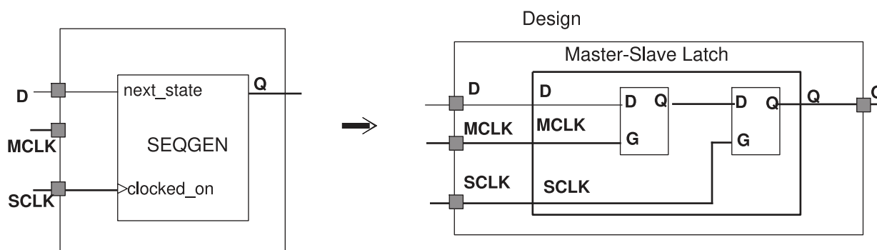
Figure 94 Generic Cell and Master-Slave Latch After Compilation
