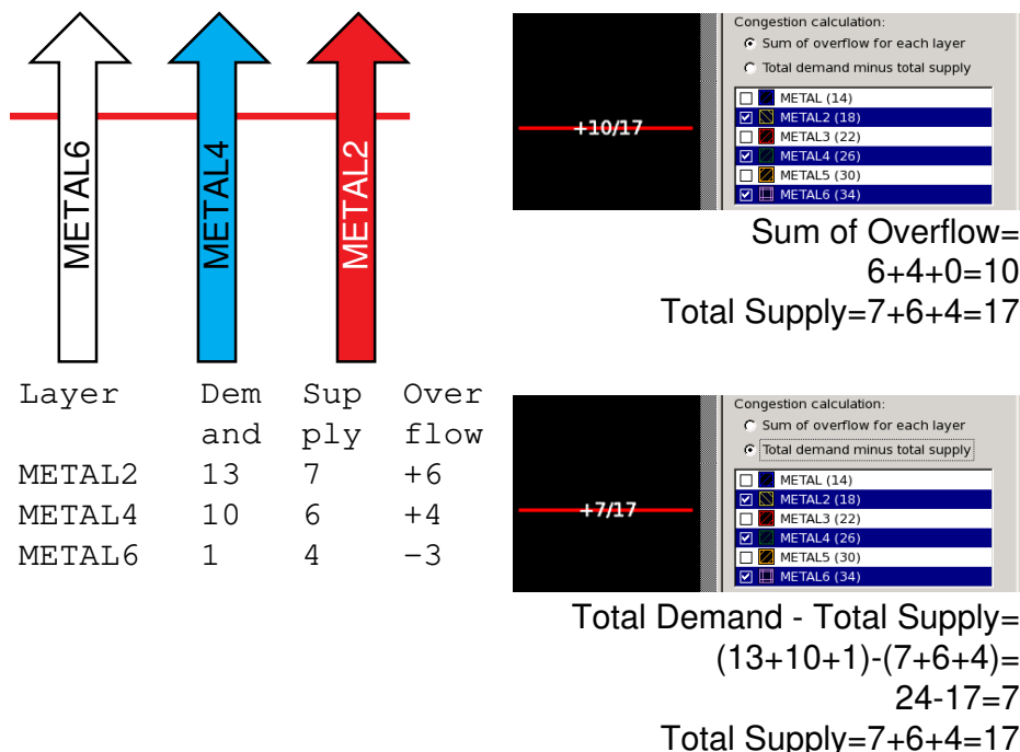
Figure 154 Congestion Example
