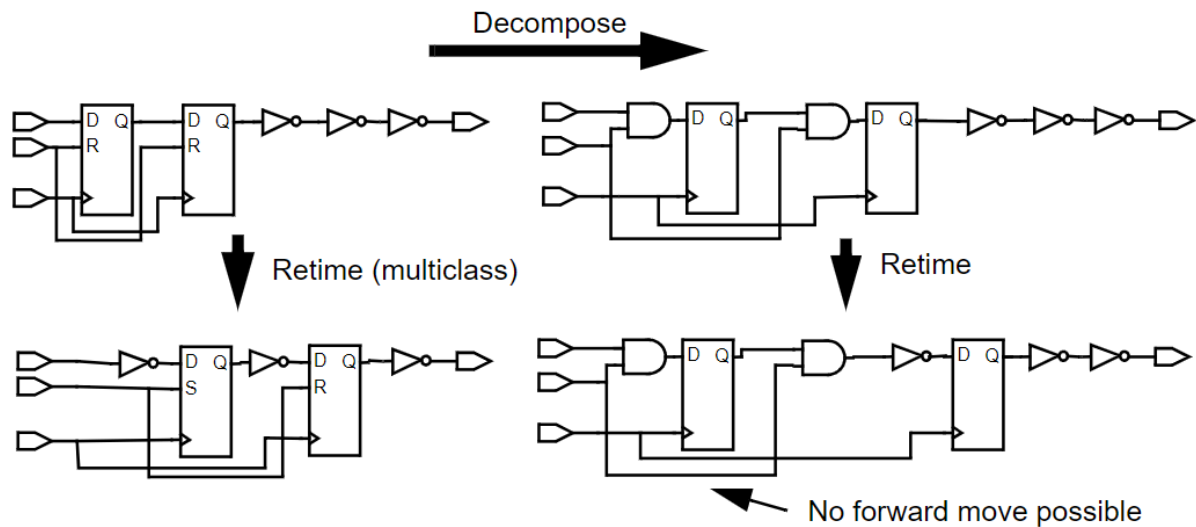
Figure 145 Reduced Mobility After Decomposition
