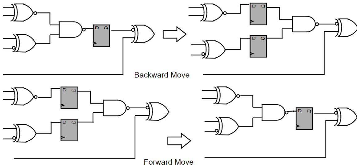
Figure 128 Adaptive Retiming
