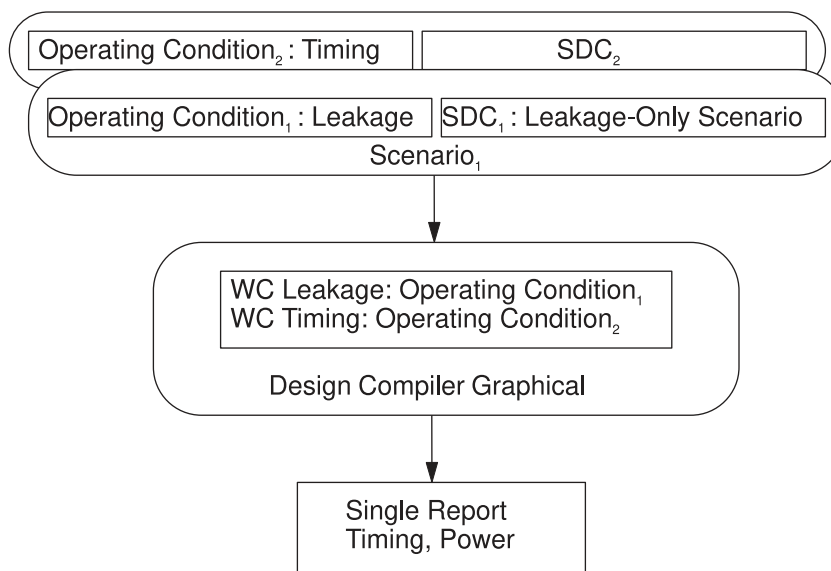
Figure 165 Setting Different Constraints on Different Scenarios
