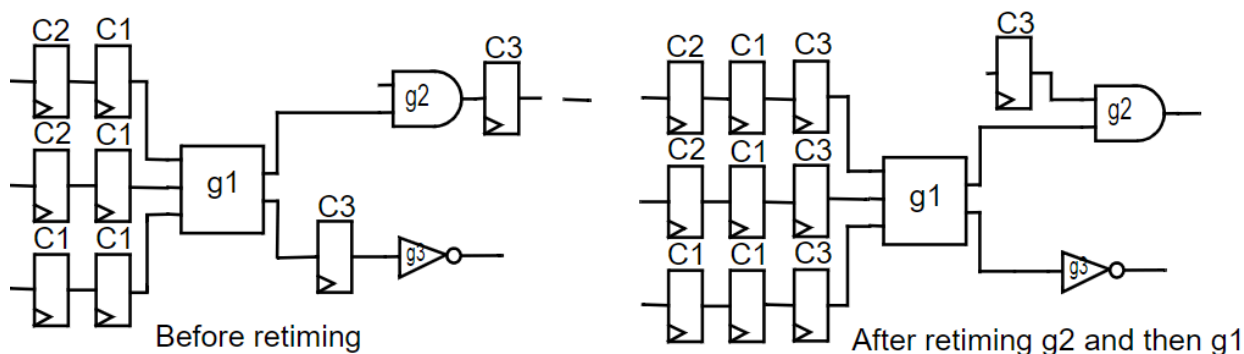
Figure 138 Backward Retiming Example
