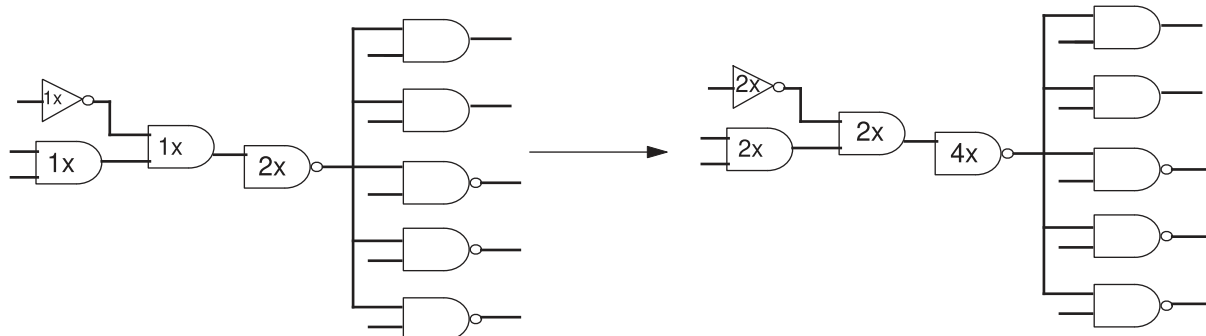
Figure 147 Delay Optimization Steps
