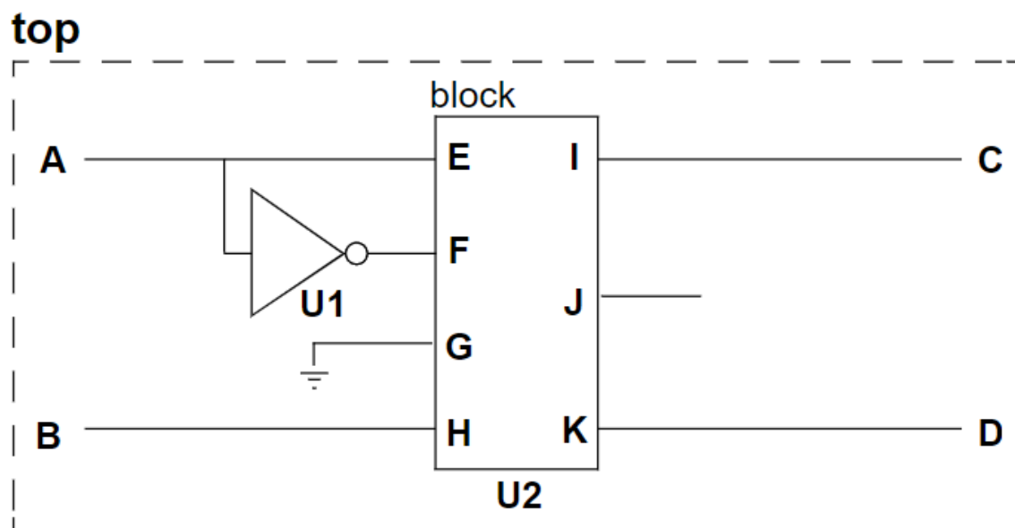
Figure 44 Characterizing Port Connection Attributes
