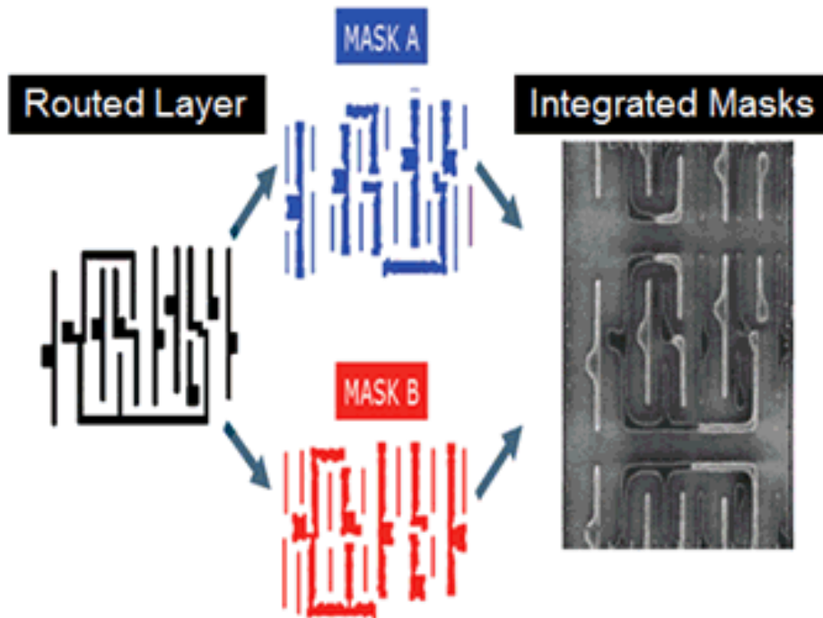
Figure 169 Double-Patterning Example
