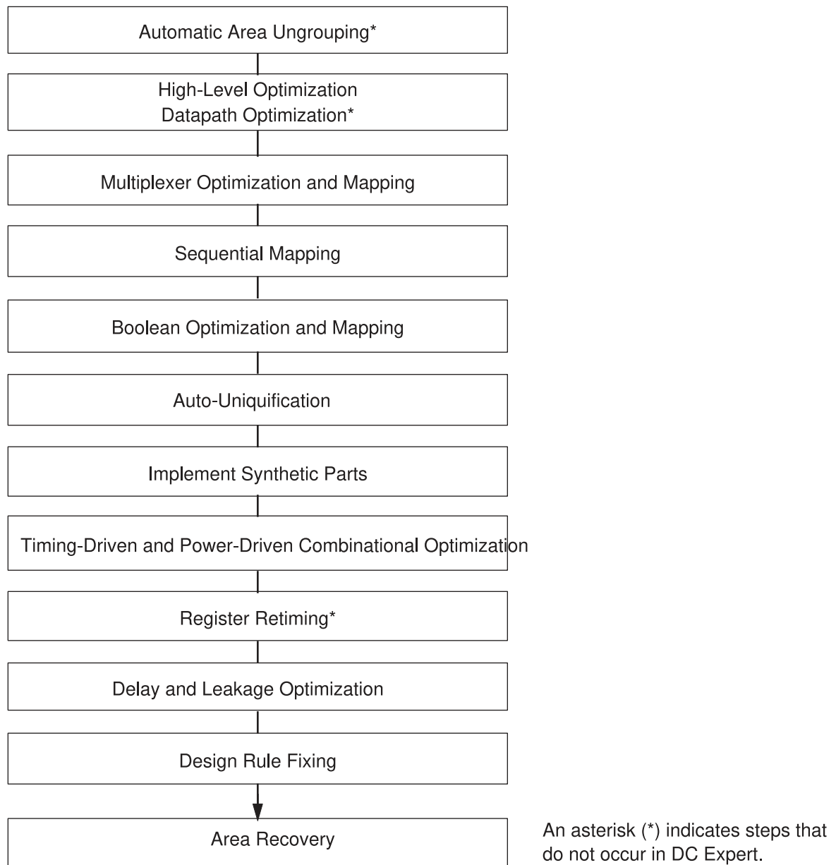
Figure 85 Optimization Flow
