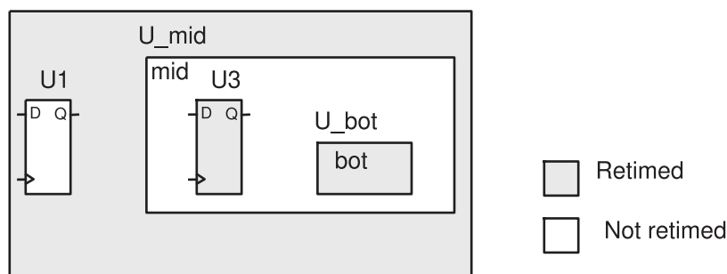
Figure 144 Cells U1 and Design mid Are Not Retimed
