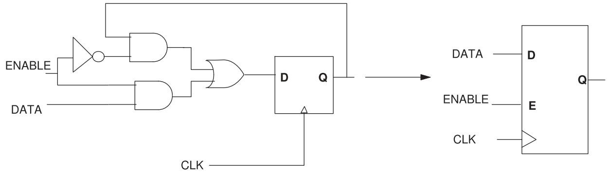
Figure 83 Sequential Optimization
