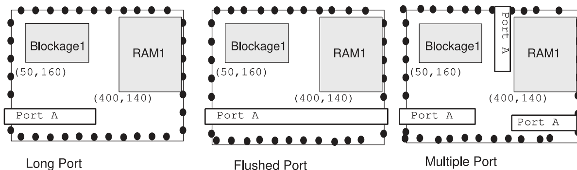
Figure 50 Types of Port Dimension Specifications
