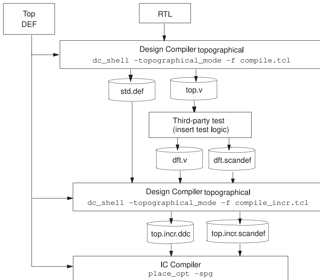
Figure 155 Physical Guidance Third-Party Test Flow
