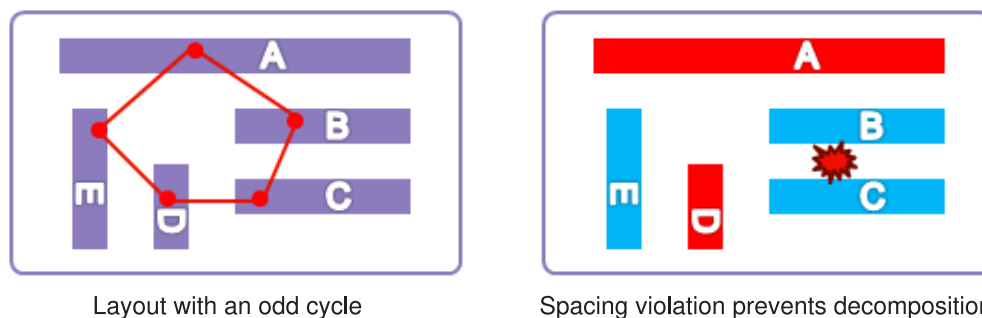
Figure 170 Odd-Cycle Violation
