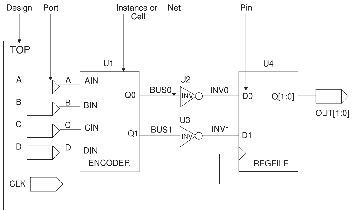
Figure 3 Design Objects
