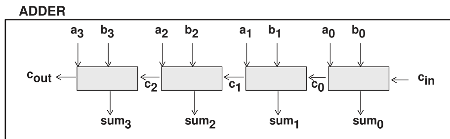
Figure 68 Hierarchical Design
