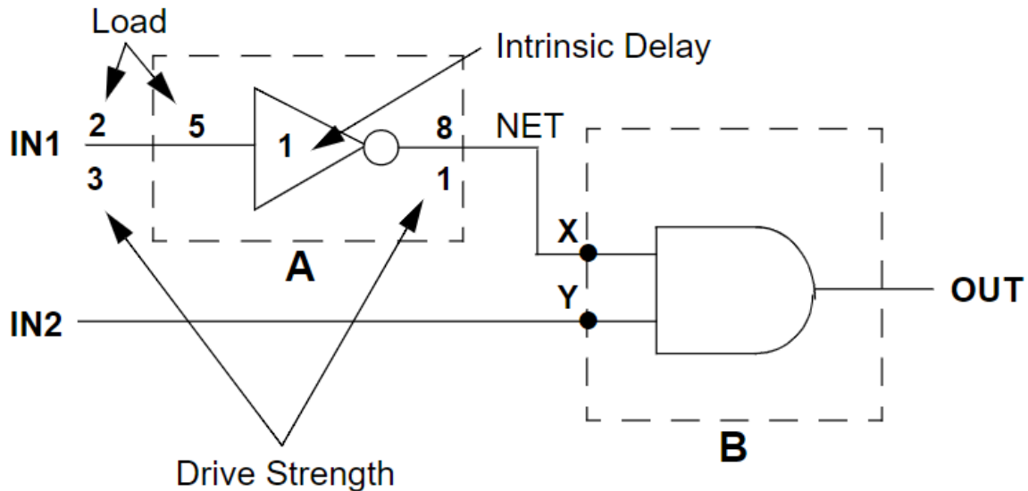
Figure 41 Design With Annotations for Timing Calculations
