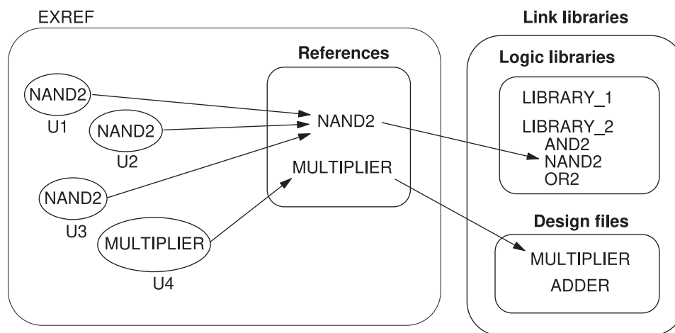
Figure 20 Resolving References
