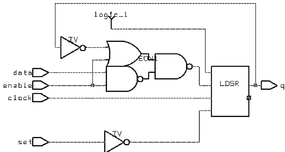
Figure 194 Synthesized Design for D Latch With Enable and Asynchronous Set
