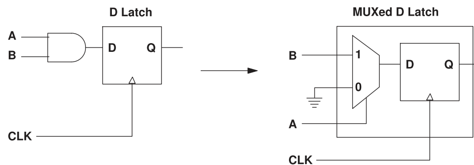
Figure 82 Sequential Optimization
