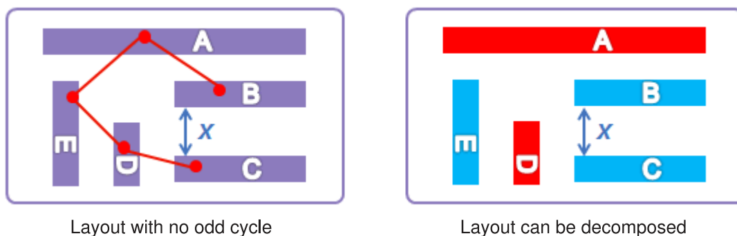
Figure 171 No Odd-Cycle Violation
