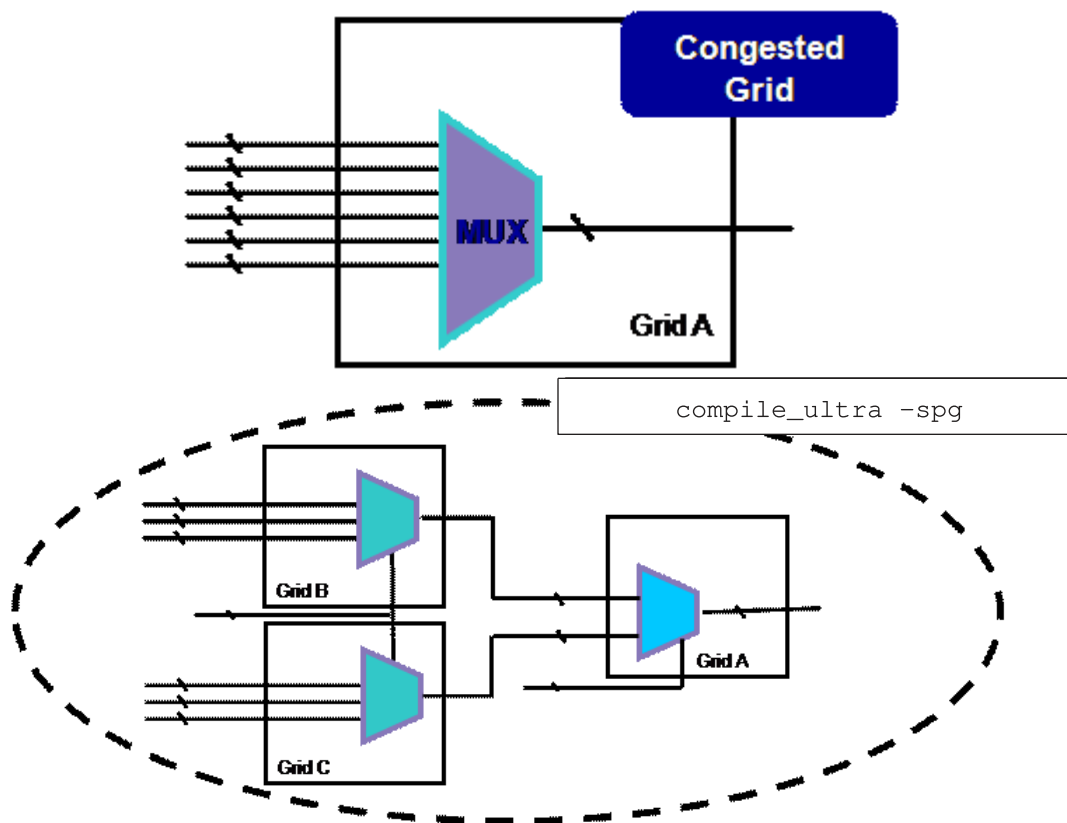
Figure 153 Optimizing RTL Structures to Minimize Congestion
