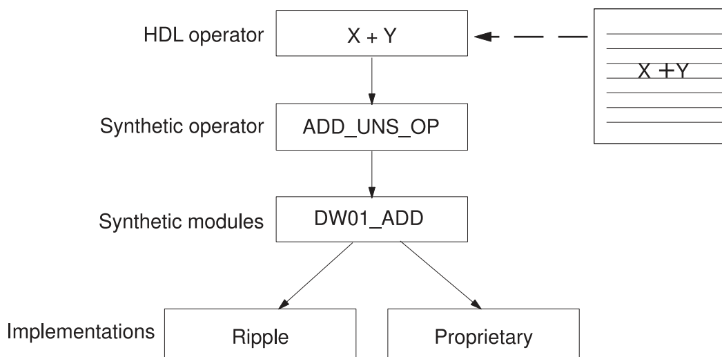
Figure 100 DesignWare Overview
