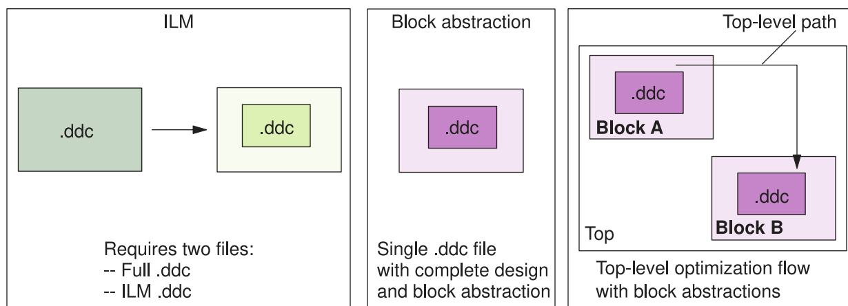
Figure 176 ILM and Block Abstraction Comparison
